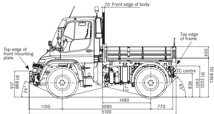
Wheelbase 3,080 mm (model variant 405.101)
